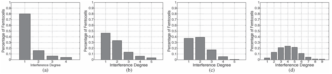
Fig. 3. Interference degree distribution for used topologies. (a) \text{SINR} = 10 dB/50 FAPs. (b) \text{SINR} = 25 dB/50 FAPs. (c) \text{SINR} = 10 dB/200 FAPs. (d) \text{SINR} = 25 dB/200 FAPs.
