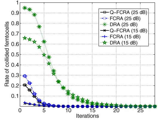
Fig. 13. Convergence time of Q-FCRA, FCRA, and DRA methods in high-density networks.
