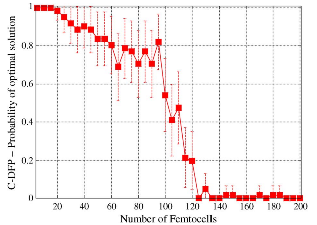
Fig. 6. Probability of finding the optimal solution for the centralized approach, i.e., \text{SINR} = 25 dB.
