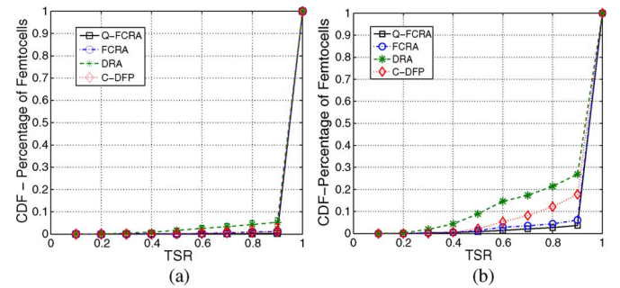
Fig. 5. CDF of TSR in low-density networks. (a) \text{SINR} = 10 dB. (b) \text{SINR} = 25 dB.
