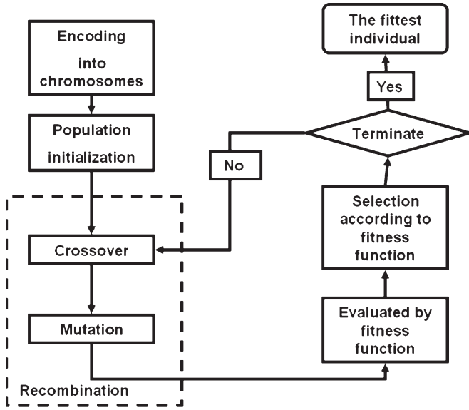
Fig. 6. Flowchart of the proposed GA.
