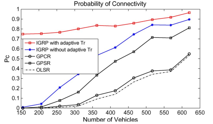
Fig. 10. Connectivity probability.
