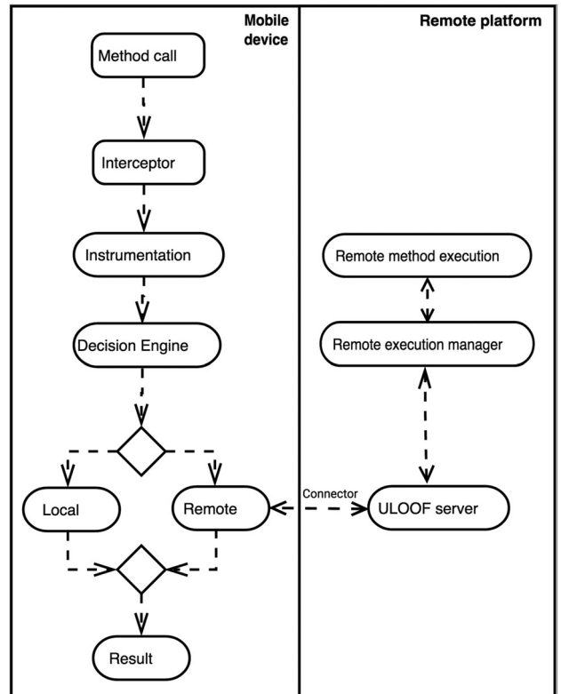
Fig. 2. Diagram of the ULOOF offloading framework modules. Authorized licensed use limited to: Bibliothèque ÉTS. Downloaded on November 18, 2025 at 18:18:32 UTC from IEEE Xplore. Restrictions apply.
