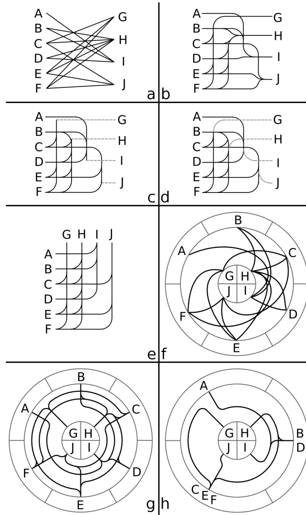
Figure 2: The same bipartite graph shown in different ways. (a) Status-quo approach. (b) Each edge starting on the left leads to a vertical bundle, and each vertical bundle leads to a single node on the right. (c,d) Variations on (b) that make the connections from vertical bundle to node on the right more visually distinct. (e) A variation inspired by Figure 3 in [7], where each node on the left corresponds to a horizontal bundle, and each node on the top corresponds to a vertical bundle. (f) A radial layout with a naïve way of drawing edges that scales poorly. (g) An improved way of drawing edges: each edge starting on an outer node leads to a circular bundle, and each circular bundle leads to a single inner node. (h) A further improvement that groups together nodes having the same neighbors.
