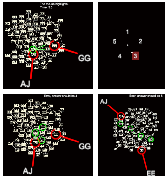
Fig. 2. In study 1, in the VR2DHilite condition, the user can move the mouse cursor over a node, causing incident edges to highlight in green (Top Left). Once the user has determined the distance in edges between the two nodes indicated in red (AJ and GG), they hold down the trigger button with their non-dominant hand (NDH), causing a radial menu to appear (Top Right). By tilting their hand down and right, they select “3” in the menu, and then release the trigger button to complete their answer. In this example, their answer is wrong, so the system displays error feedback: a correct shortest path of length 4 is highlighted (Bottom Left). Another example of error feedback (Bottom Right) is for the network shown in Fig. 1 (Left), where the shortest path has length 5.
