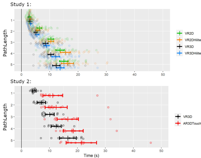
Fig. 10. Duration of trials.
