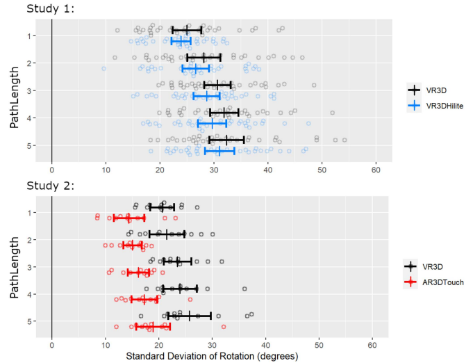
Fig. 11. How much users rotated their view of the network (Section IV-G).
