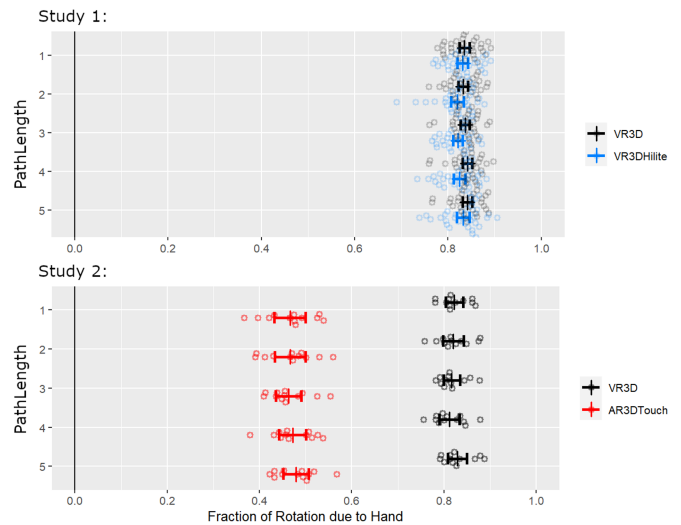
Fig. 12. How much of the rotation was due to hand motion, as opposed to head motion (Section IV-G).
