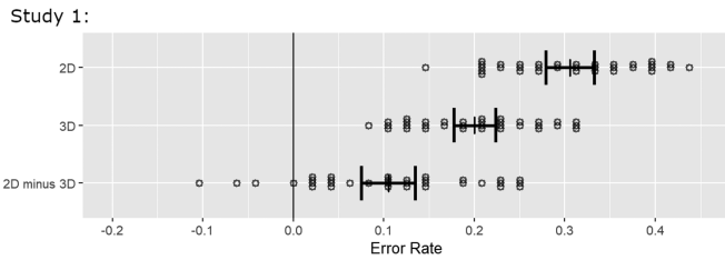
Fig. 5. Error rates in study 1, excluding PathLength 1 and 5. “2D” is the union of VR2D and VR2DHilite; “3D” is the union of VR3D and VR3DHilite. Each dot is the average for one user, and the bars show 95% confidence intervals (CIs), computed from the 34 users. A paired t -test yields p < 0.0000005 . The 3D conditions resulted in a lower error rate than 2D, confirming the first of our preregistered predictions.
