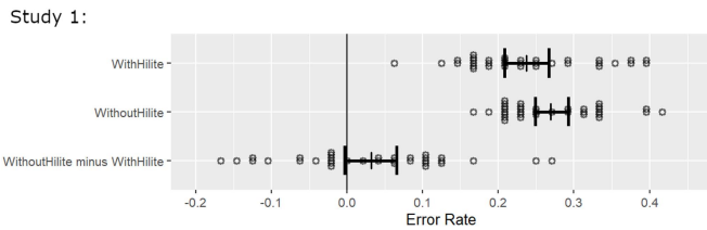
Fig. 6. Error rates in study 1, excluding PathLength 1 and 5. “WithHilite” is the union of VR2DHilite and VR3DHilite; “WithoutHilite” is the union of VR2D and VR3D. A paired t -test yields p < 0.09 , providing limited evidence of our second preregistered prediction, that the mouse improves error rates.
