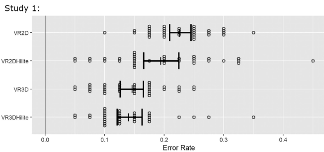
Fig. 7. Error rates in study 1 by MainCondition , including all PathLength values 1-5.
