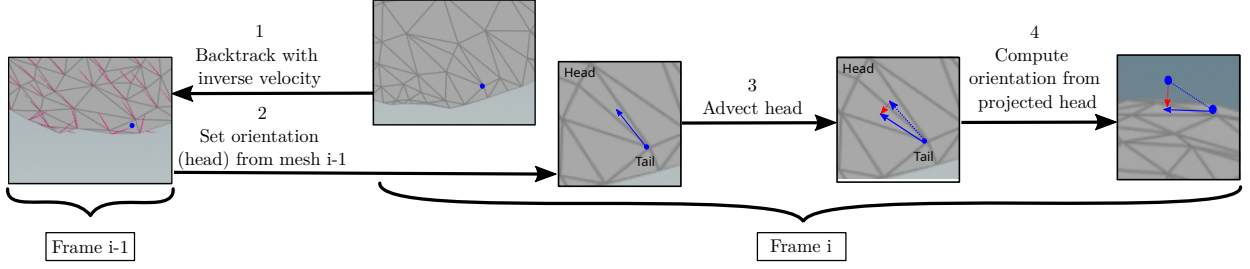
Figure 4: Advection of the orientation field by backtracking to the position on the previous frame.
