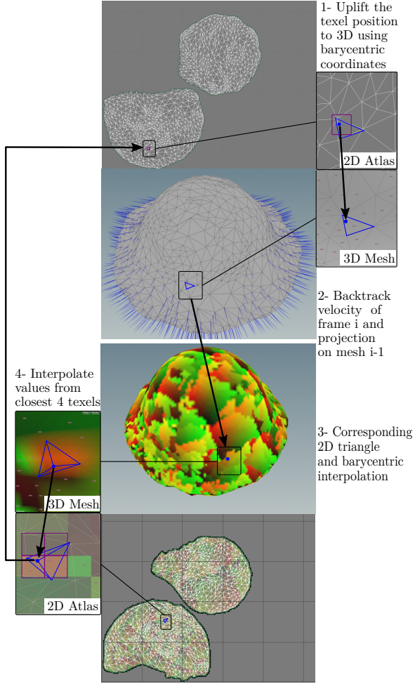
Figure 3: UV coordinates of a current frame i are computed by backtracking to the previous frame based on the velocity field.
