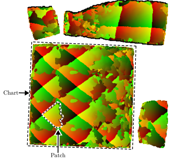
Figure 6: A typical atlas with what we refer to as charts (separate parts of the mesh flattened to 2D) and patches (contiguous group of texels with smoothly varying UV coordinates).
