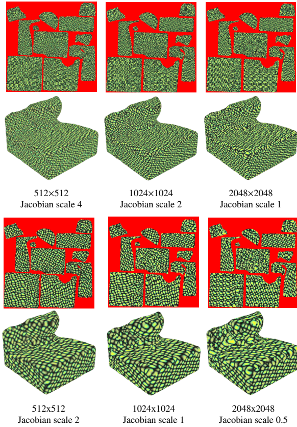
Figure 12: Synthesis results using atlases at different resolutions. The first and third rows show the texture atlases, while the second and fourth rows show the rendered fluid surfaces.
