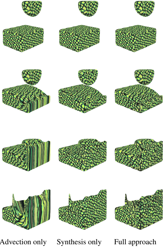
Figure 13: Ablation study results showing texture synthesis on fluid simulation over time. Left: When only relying on advection we see significant stretching. Middle: Only synthesis variant, showing good texture details but suffering from temporal incoherence (see accompanying video). Right: Our adaptive approach, which combines advection and synthesis to produce good fidelity and temporal continuity. The figure shows selected frames from an animation, in temporal order from top to bottom. Note that all variants begin from the same first frame.
