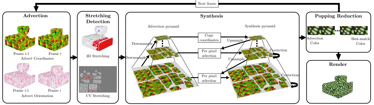
Figure 2: Pipeline of our approach. The synthesized UV coordinates are mapped to the red and green channels for depiction (boxes corresponding to advection and synthesis).
