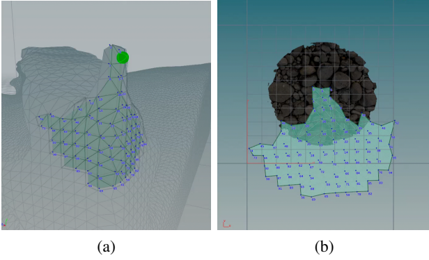
Figure 6: Patch in 3D (a), where the corresponding patch center p in the uv domain (b) is very close to the patch boundary edges.
