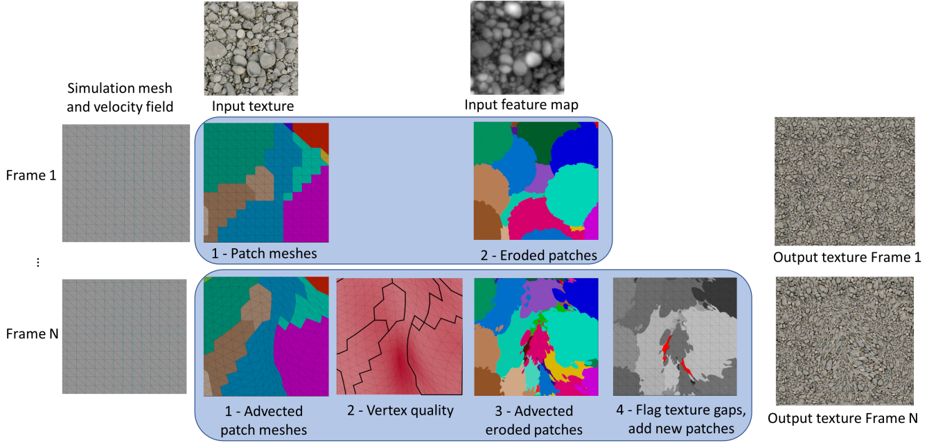
Figure 2: Overview of our approach.
